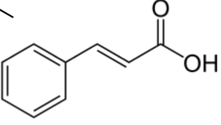
Cinnamic acid
